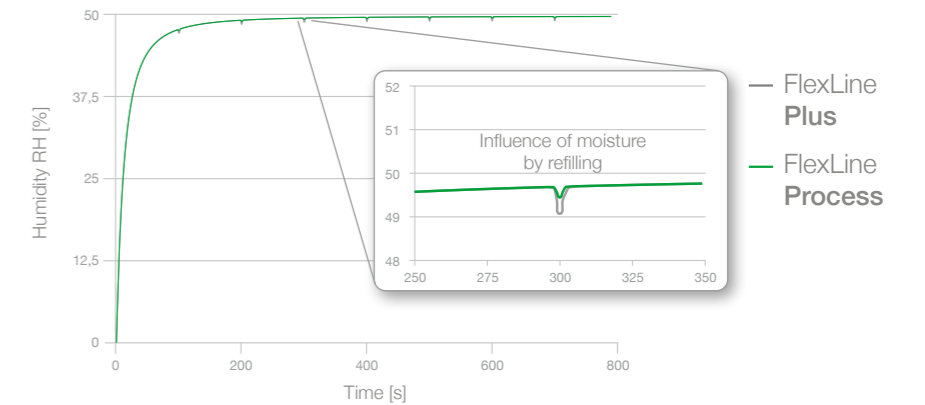
Moisture profile in operation with purified water *
